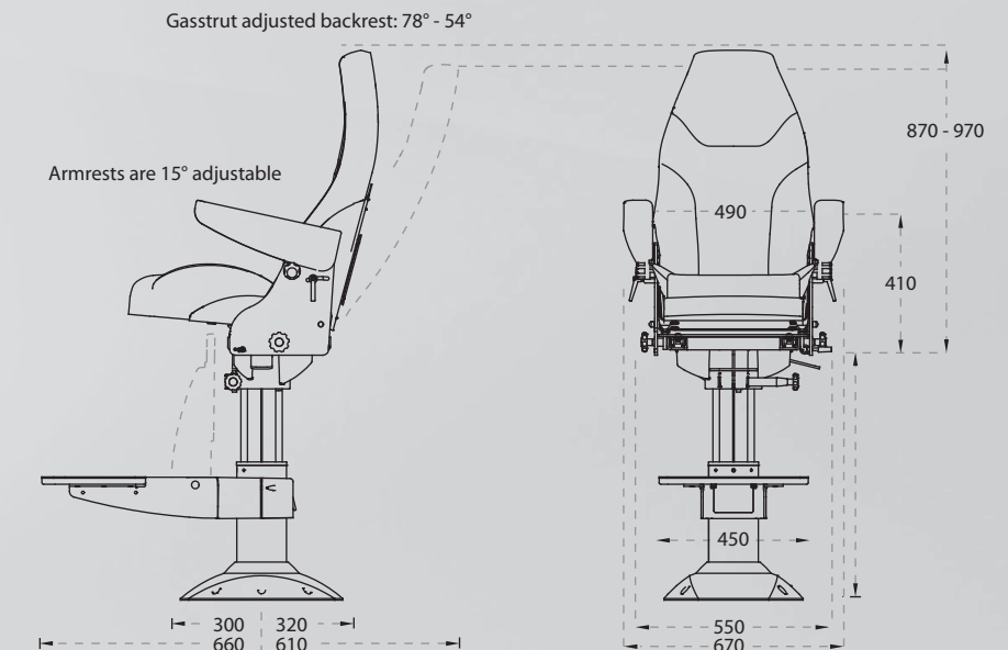
Working diameter of the chair folded Ø820. Expanded, Ø134. Weight 50 Kg.
