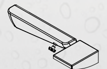
5907H (right) / 5907V (left) W=200 mm 5912H (right) / 5912V (left) W=250 mm Armrest fitting for combining mouse trackball and joystick. *Joystick not supplied
