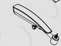
5804H (right) / 5804V (left) Armrest with casing Ø60 for small joystick. *Joystick not supplied
